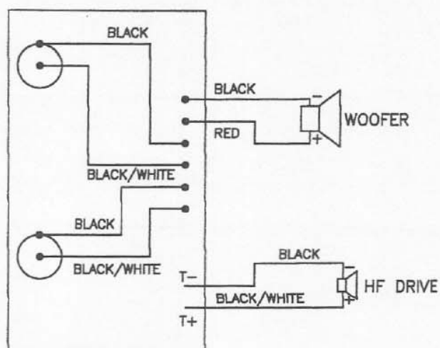
WIRING DIAGRAM
