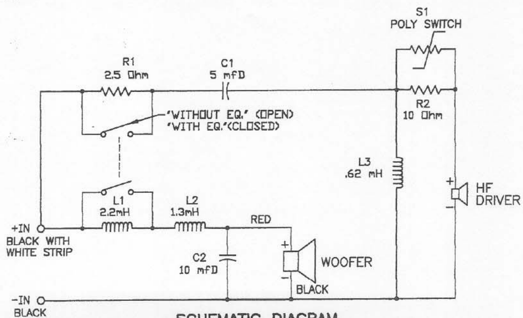
SCHEMATIC DIAGRAM CROSSOVER FOR 200S (P/N 82909)
